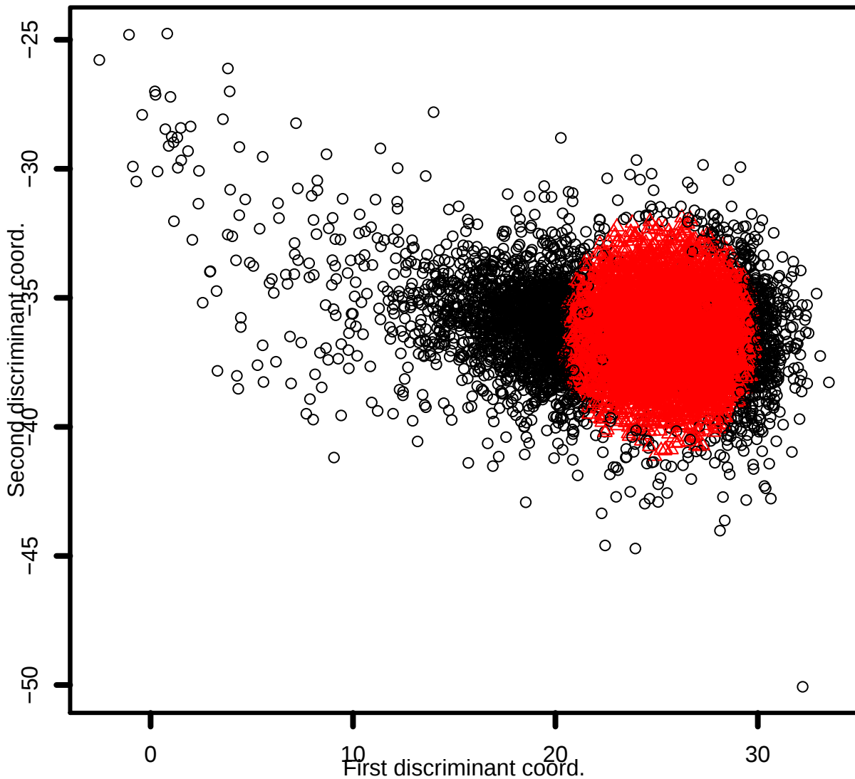
pbmc8k (n= 8707 ) cells clustering by gene body coverage k = 1, \alpha = 0.3
